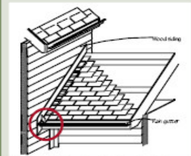
Kick-out flashing (seen in the red circle) diverts water away from the wall and into the gutter.
